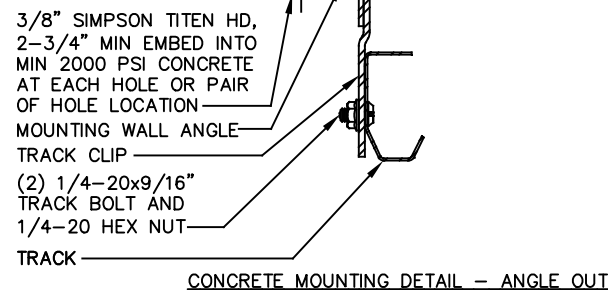
CONCRETE MOUNTING DETAIL - ANGLE OUT
