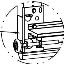
DETAIL E
